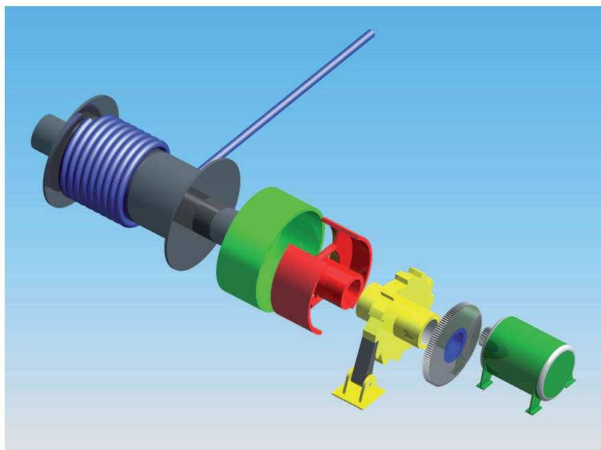
Fig. 6: Schematic exploded view of components SafeWinch
