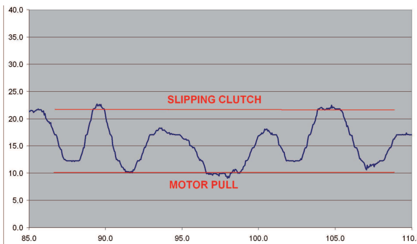
Top: Fig. 10: Dynamic sea tests, SafeWinch cuts off peak loads and prevents slack wire Middle: Fig. 11: Towline load measurements (Clutch 32 / Pull 10 ton) Bottom: Fig. 12: Towline load measurements (Clutch 22 / Pull 10 ton)
